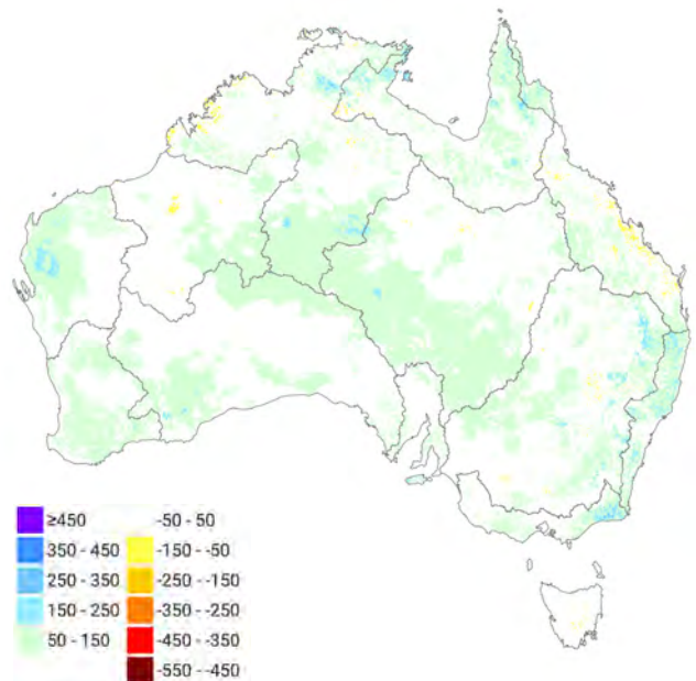
Soil moisture change from previous year (mm)
