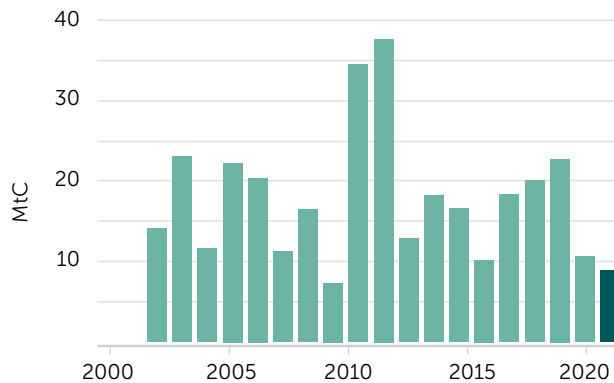
National Carbon emissions from fire
